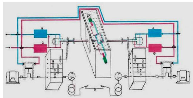
Project device SaDaM-2
