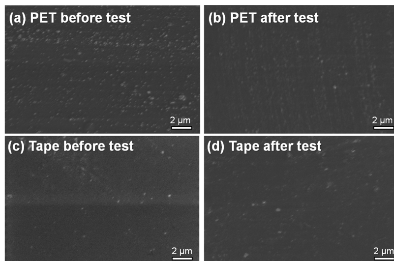
Figure 11. SEM images of PET (a) before and (b) after endurance test and double-sided tape (c) before and (d) after endurance test at 20,000× magnification.
