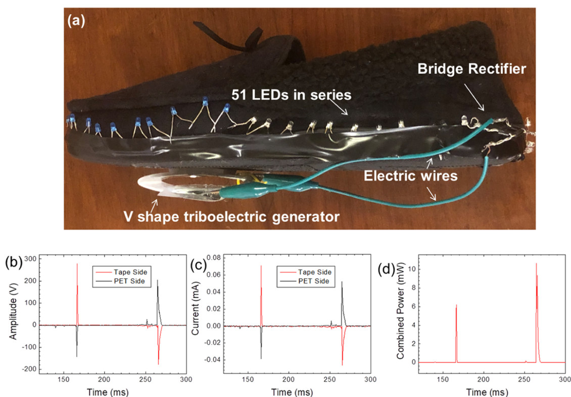
Figure 9. (a) Triboelectric generator (Al/PET/double-sided tape and PET/Al configuration) with a 38 mm × 38 mm area installed on the bottom of a shoe. A bridge rectifier circuit is used to convert AC to DC power to demonstrate the lighting up of 51 LEDs; (b) voltage; (c) current; and (d) power under a 4 MΩ electrical load.
