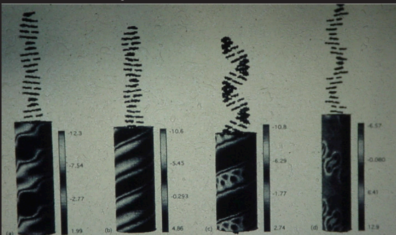
FIGURE 3. The potentials due to the bases of (a) B-DNA polyd(AT)-polyd(AT) at 11.2 Å; (b) B'-DNA polyd(A)-polyd(T) at 11.9 Å; (c) A-DNA polyd(G)-polyd(C) at 11.6 Å; and (d) Z-DNA polyd(GC)-polyd(GC) at 9.8 Å. The distances correspond to 1 Å from the charge having the largest radial coordinate in the given helix. The numbers on the scale are given in millivolts.
