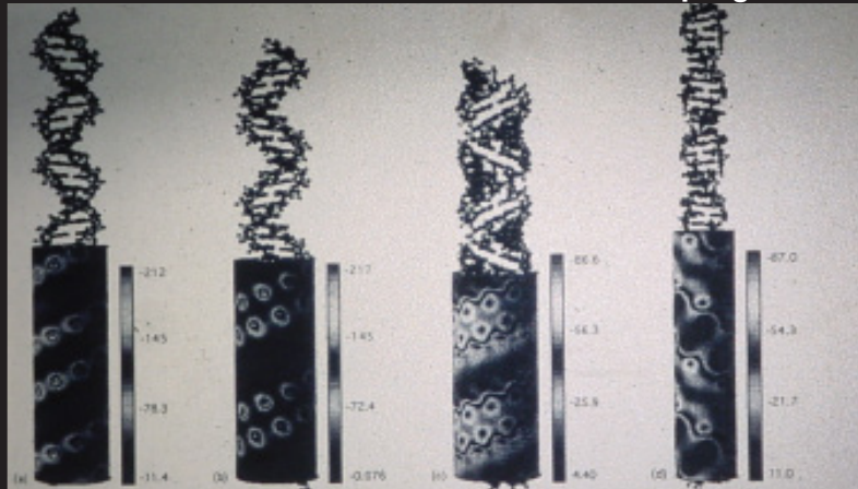
FIGURE 4. The potentials due to the double helices (a) B-DNA polyd(AT)-polyd(AT) at 11.2 Å; (b) B'-DNA polyd(A)-polyd(T) at 11.9 Å; (c) A-DNA polyd(G)-polyd(C) at 11.6 Å; and (d) Z-DNA polyd(GC)-polyd(GC) at 9.8 Å. The units of the scale are millivolts. The colored shells are located as regions from the charge of the helix with the largest radial coordinate.
