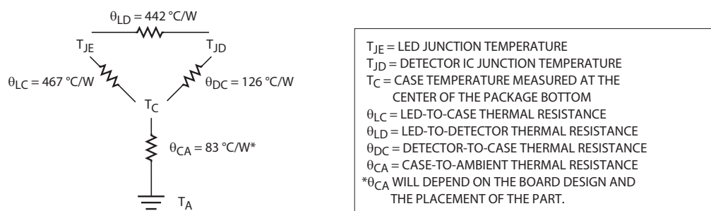
Figure 28 Thermal Model
