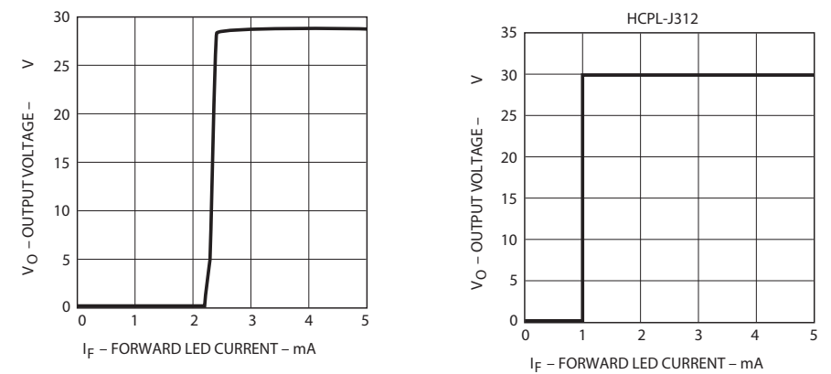
Figure 15 Transfer Characteristics
