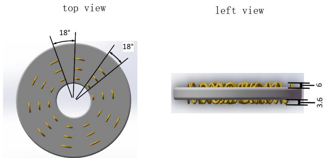
Figure 9 Parameters of coils winding
