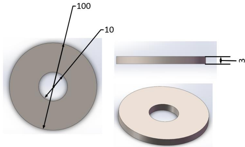
Figure 12 Iron core
