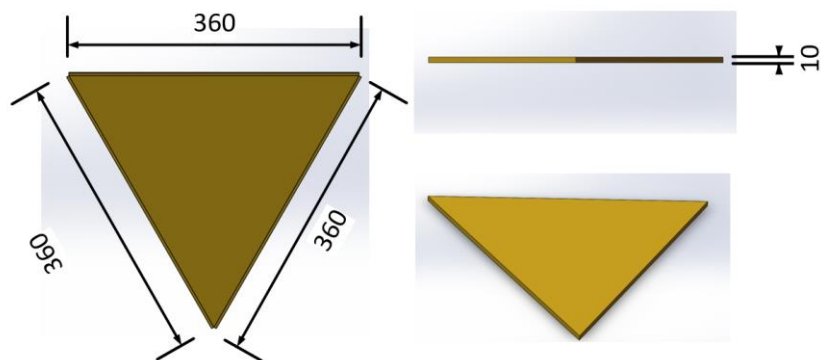
Figure 18 Size of triangle plate
