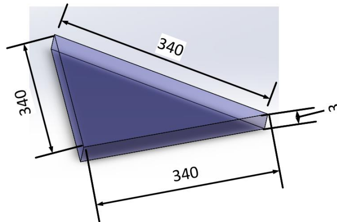
Figure 14 Size of triangle
