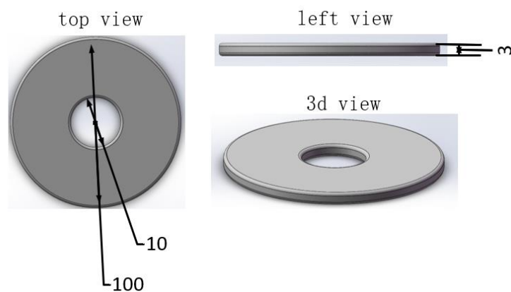
Figure 11 Size of round plate
