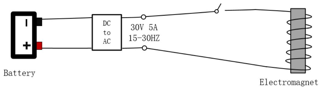
Figure 23 Circuit diagram of the device
