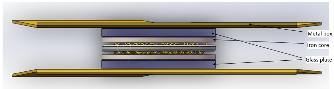
Figure 16 Position of glass plate
