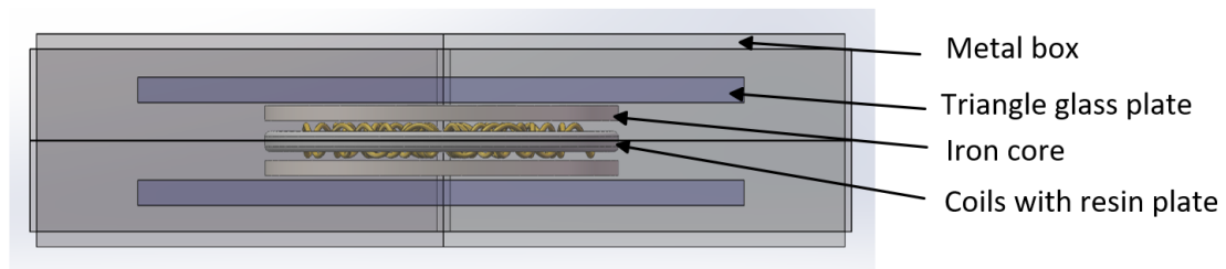
Figure 22 Positions of inside parts
