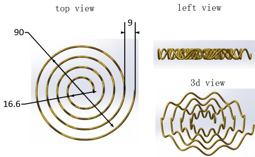
Figure 10 Magnet coils
