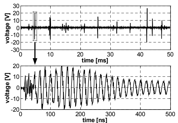
Fig. 17: Measured output voltage at the load
