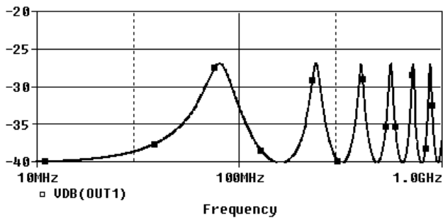
Fig. 8: Power transfer of a transmission line transformer
