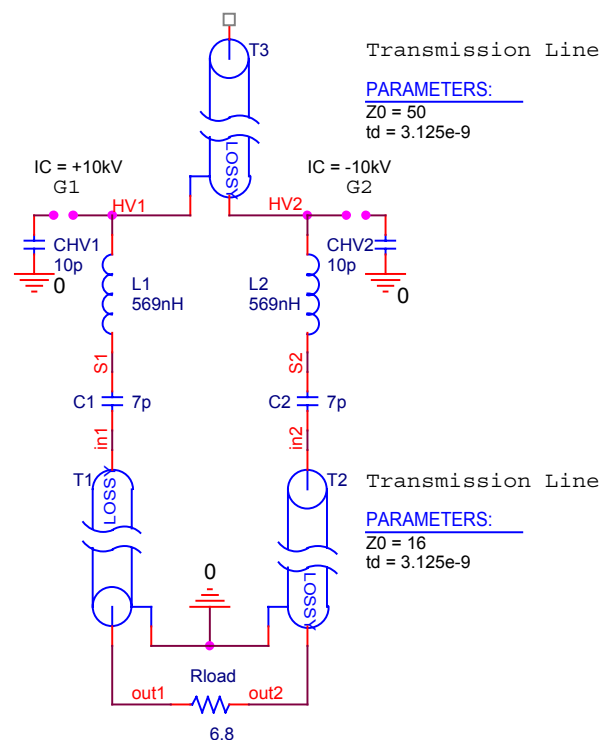
Fig. 11: Circuit of the complete push-pull transformation device
