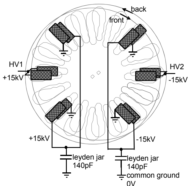
Fig. 3: Configuration of the electrostatic generator
