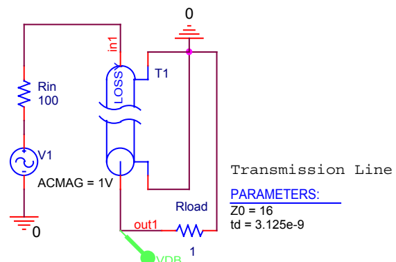
Fig. 7: Transmission line transformer
