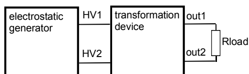
Fig. 2: Connections of the power generation system
