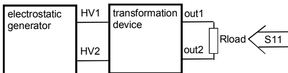
Fig. 15: Setup for resonance frequency measurement
