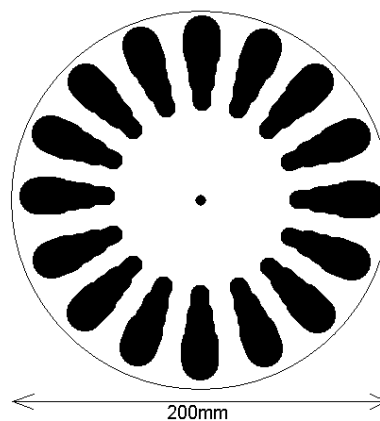
Fig. 4: Disk surface with metal sectors
