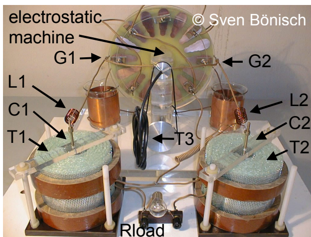
Fig. 12: Construction of the high voltage transformation system
