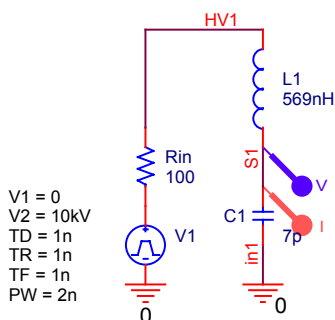
Fig. 9: Serial resonance circuit used for ESD pulse forming
