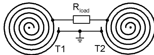
Fig. 13: Symmetrical load configuration
