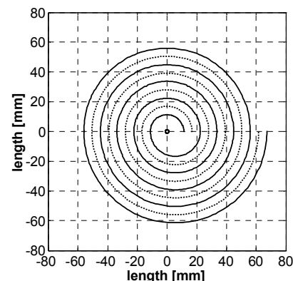
Fig. 14: Construction of the high voltage helical transmission line (one side)
