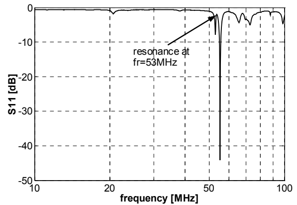
Fig. 16: Tuned resonance frequency
