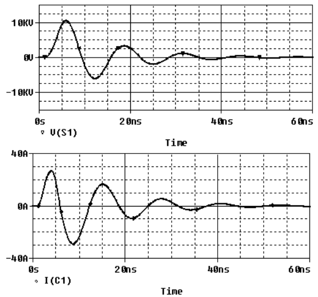
Fig. 10: Voltage and current at the pulse forming network
